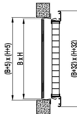
UQ21: fixing with clips
