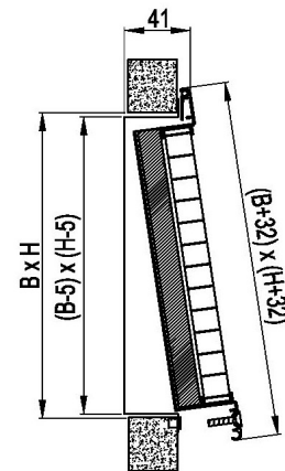
UQ13: fixing with screws
