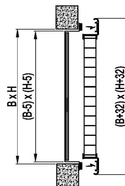
UQ22: fixing with magnets
