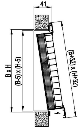
UQ12: fixing with magnets
