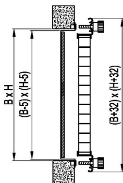
UQ24: fixing with knobs
