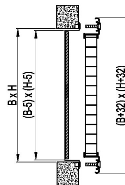
UQ23: fixing with screws
