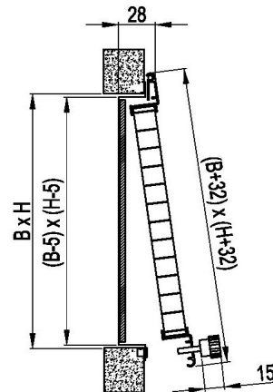
UQ3: fixing with screws
