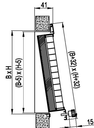
UQ14: fixing with knobs
