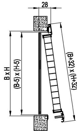
UQ3: fixing with screws
