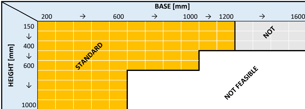
FEASIBLE SIZES - RIGID FILTER - WITH HINGE - 50mm PITCH
