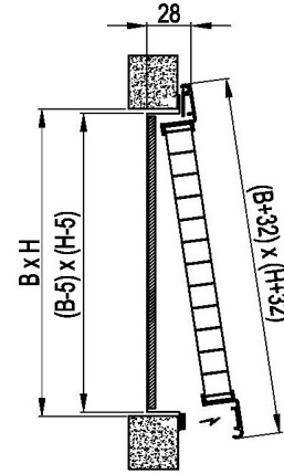
UQ2: fixing with magnets
